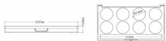
HN3426-2 Size:L145.87xW80.75xH13.08mm
