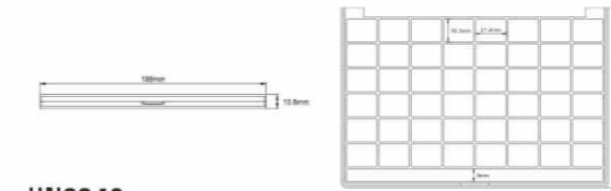
HN3348 Size:L188xW127xH10.8mm
