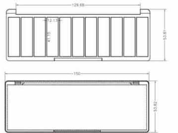
HN3479 Size:L150xW53.82mm
