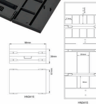
HN3415 Size:L96xW61xH38mm
