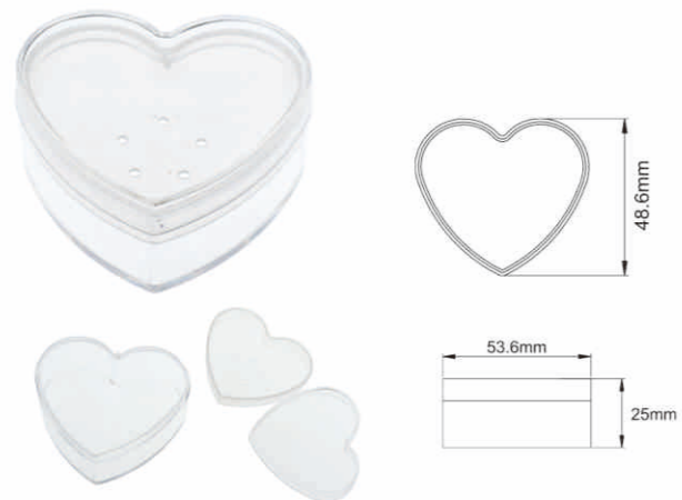
○ HN3364 Size:L53.6xW48.6xH25mm
