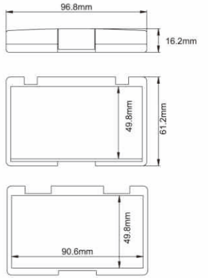
HN3414 Size:L96.8xW61.2xH16.2mm
