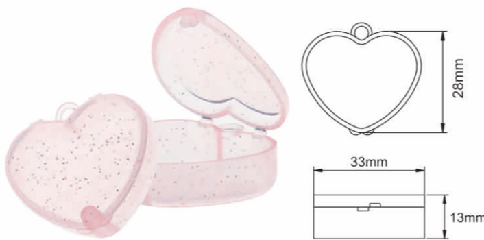
○ HN3315 Size:L33xW28xH13mm
